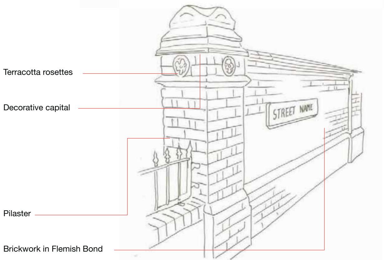
Picture 56. Front boundary wall with glazed bricks and cast iron railing
